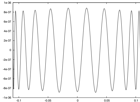
Figure 2. Absolute error between g and our polynomial
