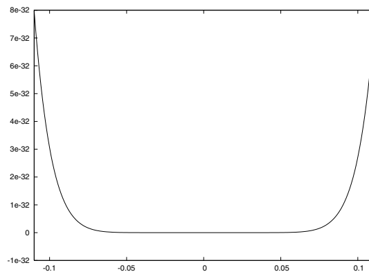
Figure 3. Absolute error between g and rounded minimax
